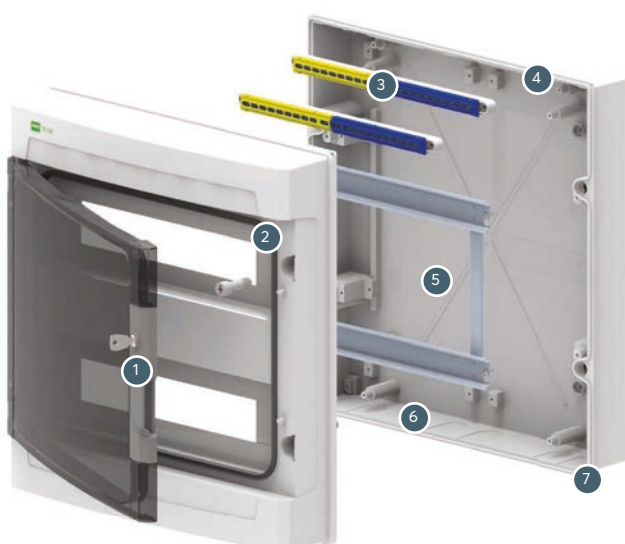
new system door locking
